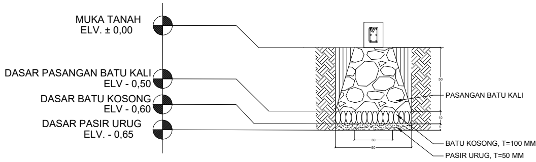
DETAIL 1 PONDASI SKALA 1:100
