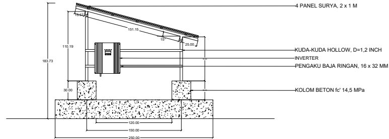
TAMPAK SAMPIING PANEL SKALA 1:30
