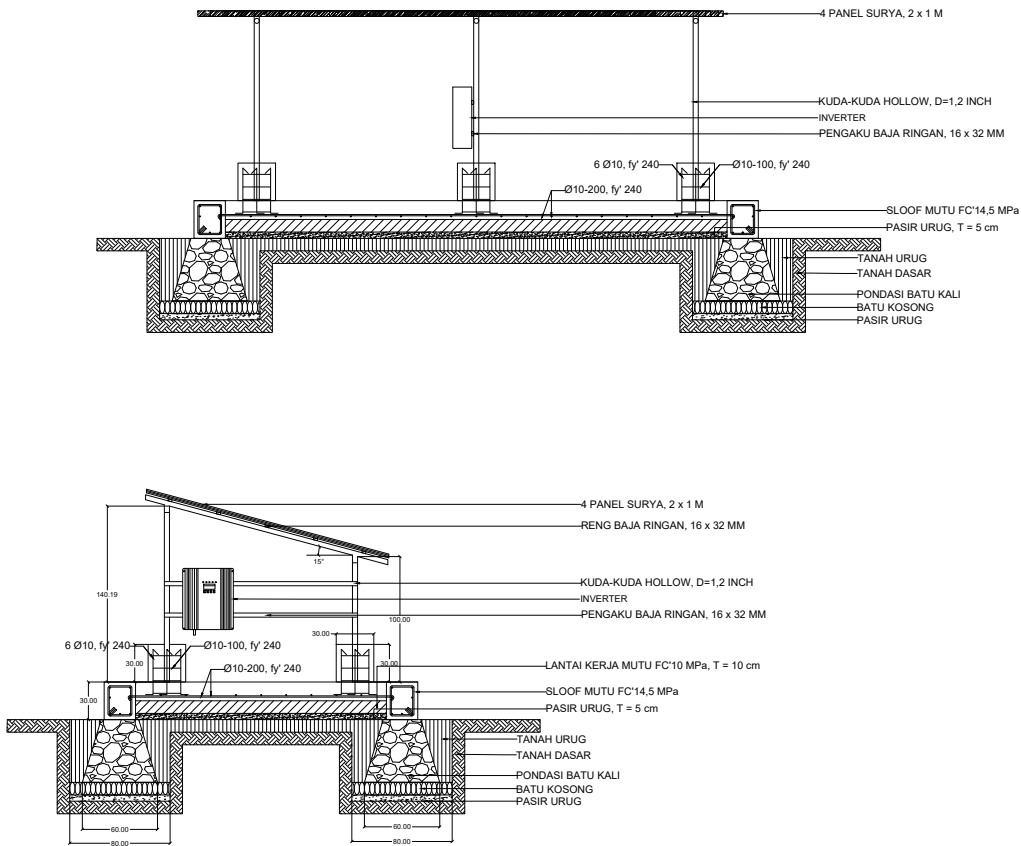
DETAIL PONDASI PANEL SURYA
